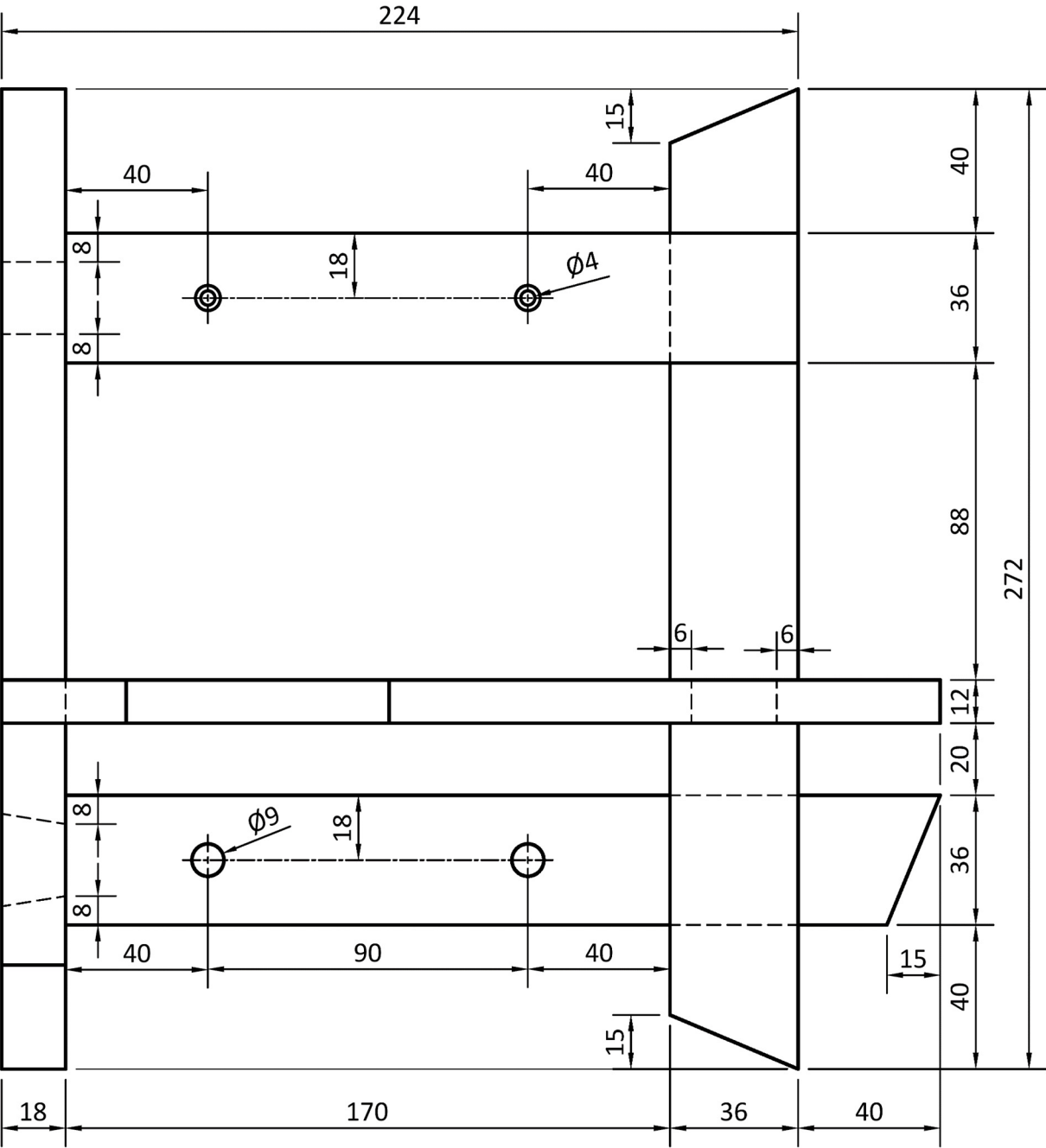
Elevation/Aghaidhchló
